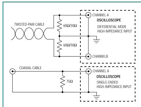
Figure 5. The upper drawing illustrates the proper way to terminate the differential transmission line, while the lower one is a termination example for single-ended transmission lines.
