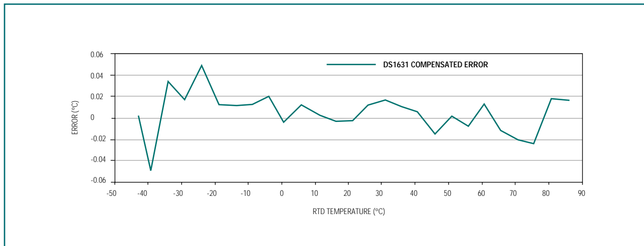
Figure 3. Compensated error provides much higher accuracy over the device's characterized temperature range than standard factory calibration.
