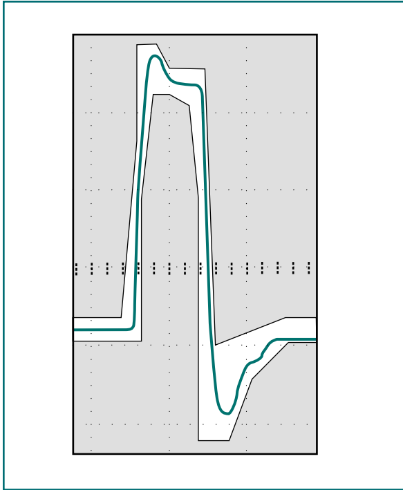
Figure 1. T1 pulse amplitude (1.544Mbps) is measured in the center of the pulse located at time T0.
