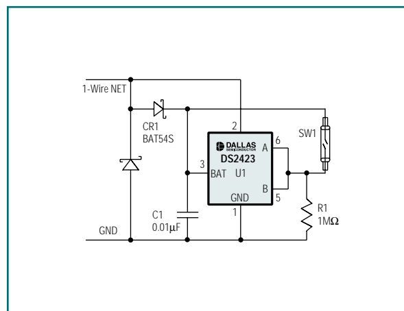
Figure 2. The basic DS2423 counter circuit uses a reed switch as an input.
