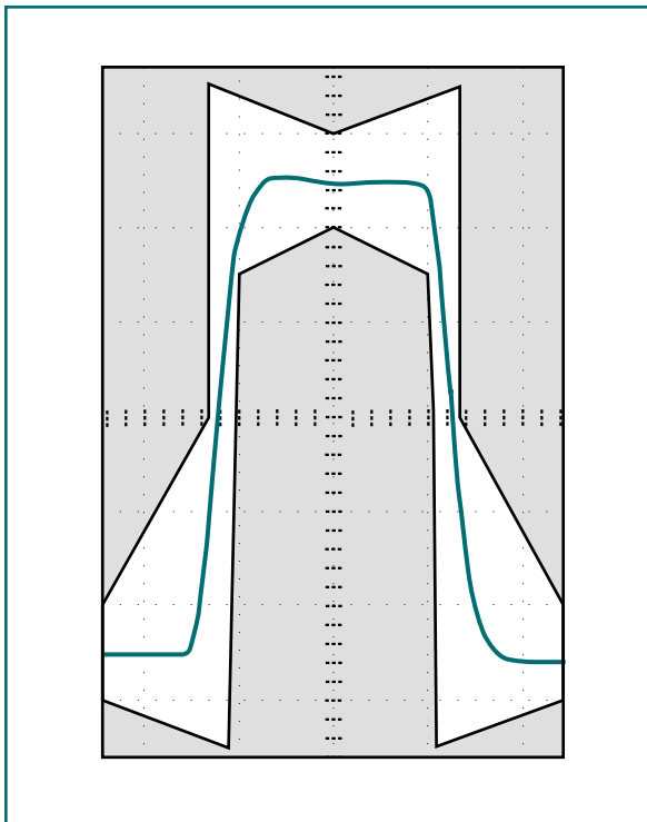
Figure 2. Every E1 pulse (2.048Mbps) must conform to the shape of the template and not just an isolated pulse.
